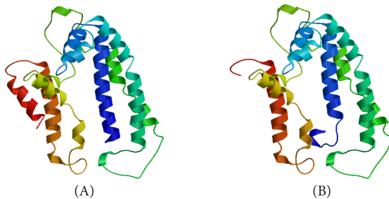
Figure 2 (A) 3D modelling of cyt b Scomberomorus commersoni ; (B) 3D modelling of cyt b Scomberomorus koreanus
